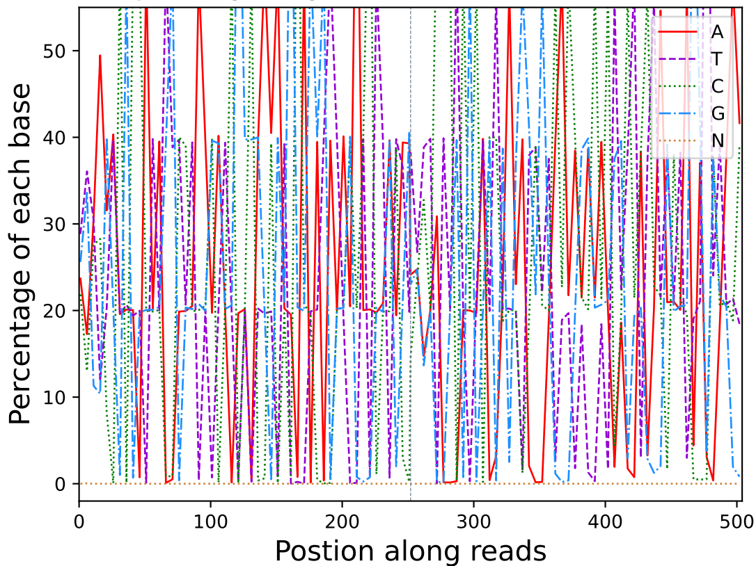
Base percentage along reads (R10227)
